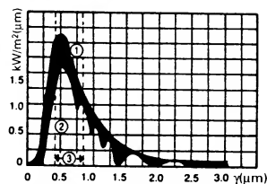
17 intensity J of solar radiation at the limit of the Earth's atmosphere as a function of the wavelength ( \gamma_s = 90^\circ ) the shaded region shows the losses from reflection, scatter and absorption of radiation due to the water vapour, carbon dioxide and ozone in the air, as well as dust particles 2 intensity J of the solar radiation that reaches the Earth 3 range of visible light
